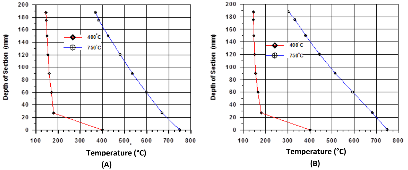
Figure 12. Temperature distributions along section depth at (A) 30mm and (B) 60mm from lateral surfaces.
