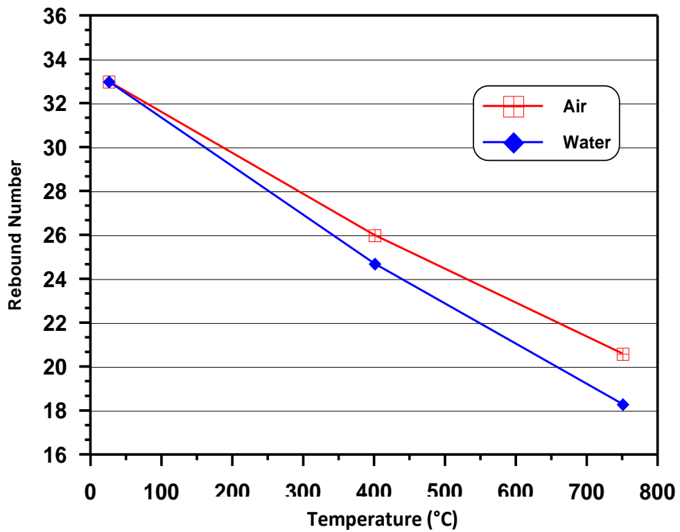
Figure 6. The effect of fire flame on the rebound number.
