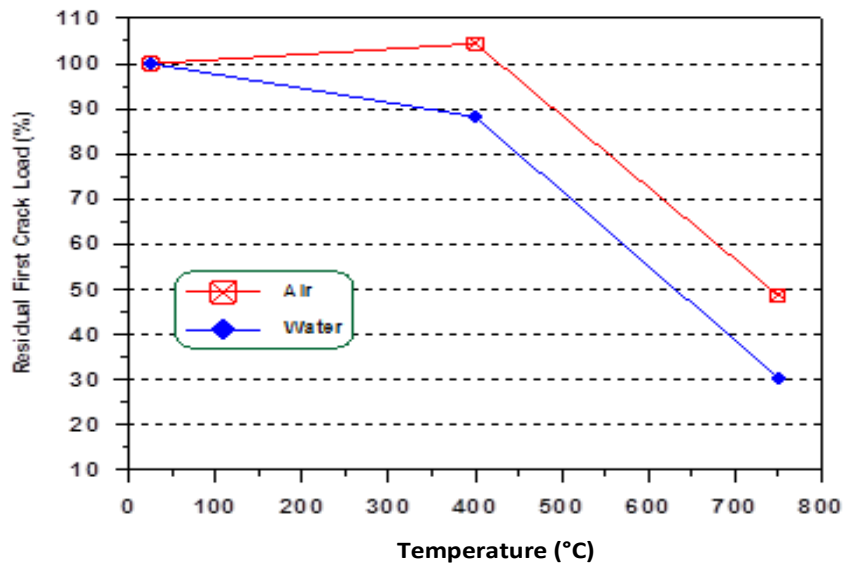
Figure 8. Effect of fire flame on the residual first crack load for the rigid beam specimens.
