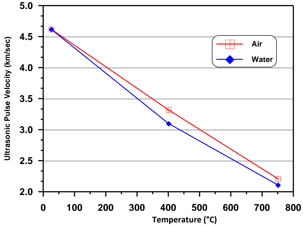
Figure 5. The effect of fire flame on the UPV.
